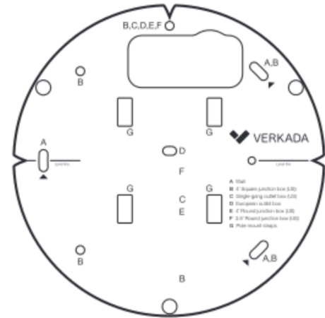
Mounting template
